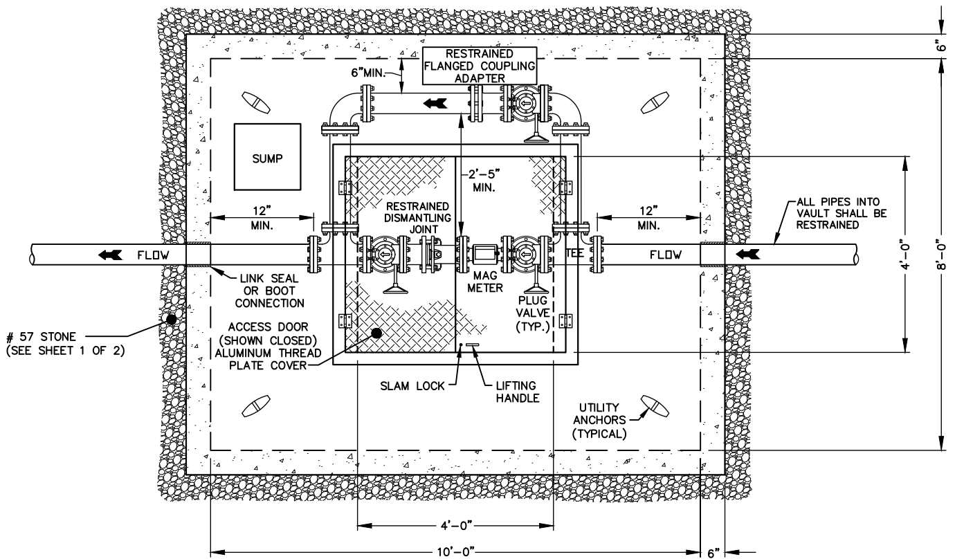
PLAN VIEW
