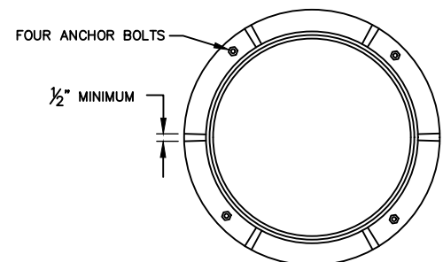
RING TOP VIEW
